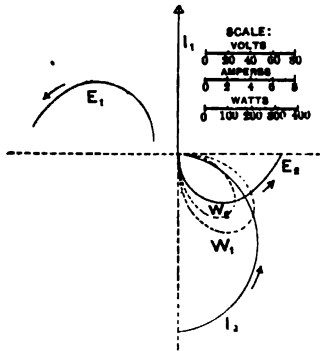
FIG. 7.—Constant Current, Step Down, Arm at 90°
